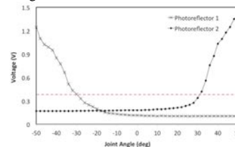
Fig. 3. Measurable joint angle range.
