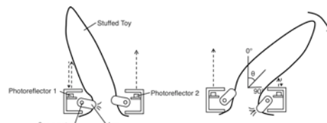
Fig. 2. Actuation principle: a pair of DC servomotors push on the toy's cover; two photoreflexors sense joint angle \theta by measuring the distance between the sensor and the cover.
